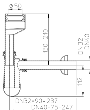
Tec. Draw. HL130
