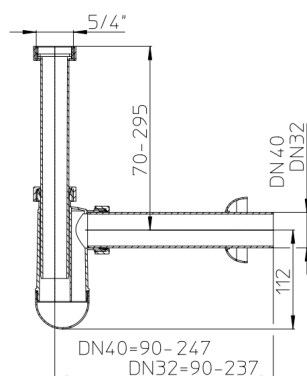
Tec. Draw. HL132
