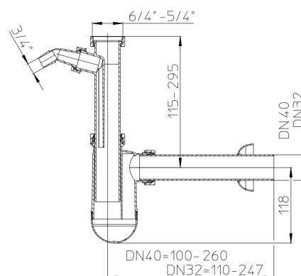
Tec. Draw. HL132.1
